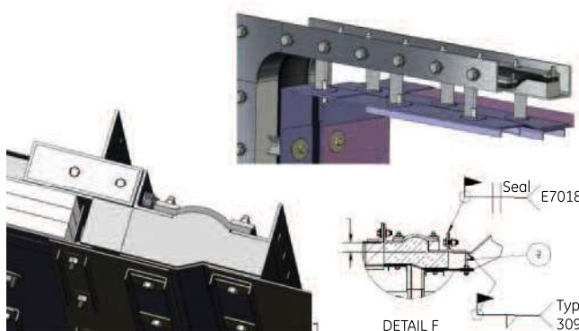
Figure 47. The advanced CHROEM designs offered by GE have an improved expansion joint.
