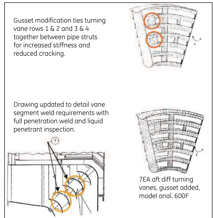
Figure 29. Cracking in CHROEM 9E aft diffuser is reduced by pipe gussets that increase stiffness of turning vanes.
