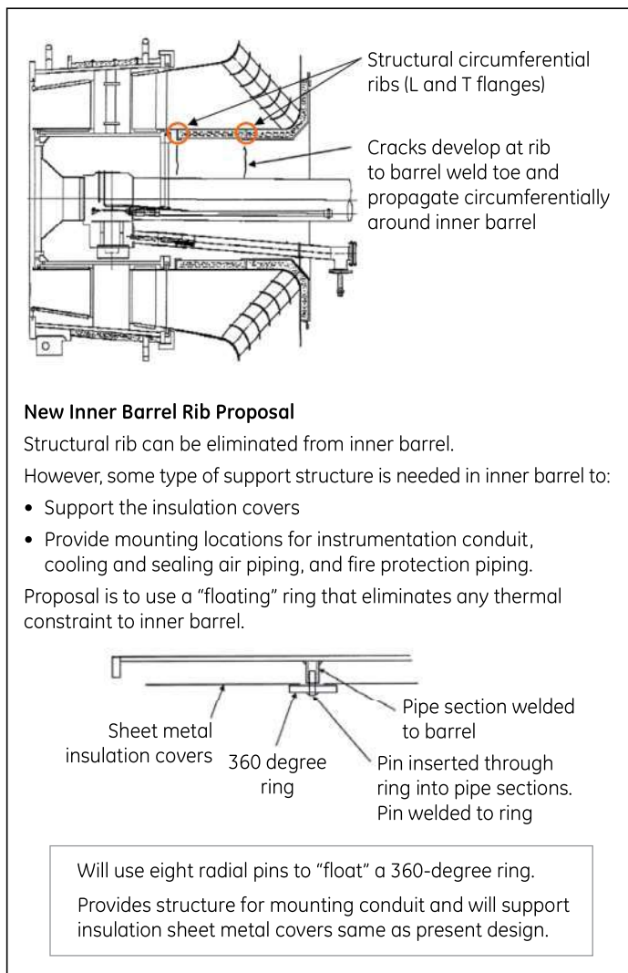
Figure 28. Elimination of structural ribs in CHROEM 9E diffuser avoids circumferential cracking in ribs.
