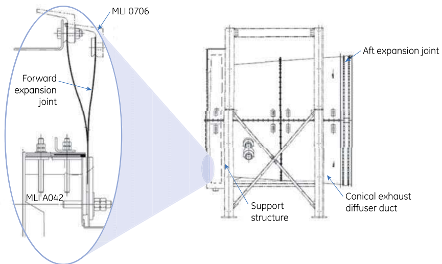
Figure 3. Typical F-Class MLI A042 arrangement.
