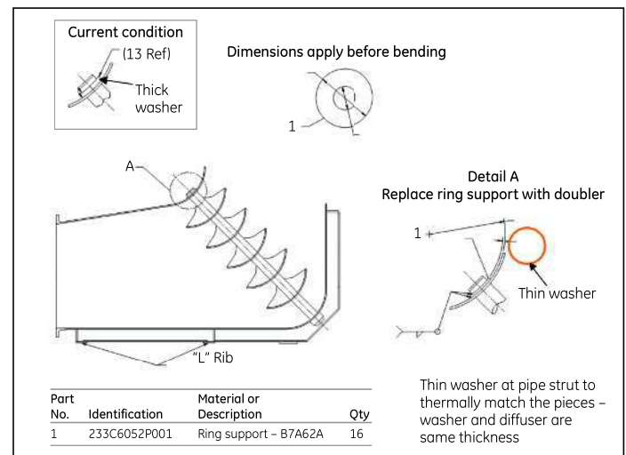
Figure 30. In CHROEM 9E aft diffuser, the washers securing turning vanes have reduced thickness to decrease thermal mismatch, lower stress, and avoid cracking.
