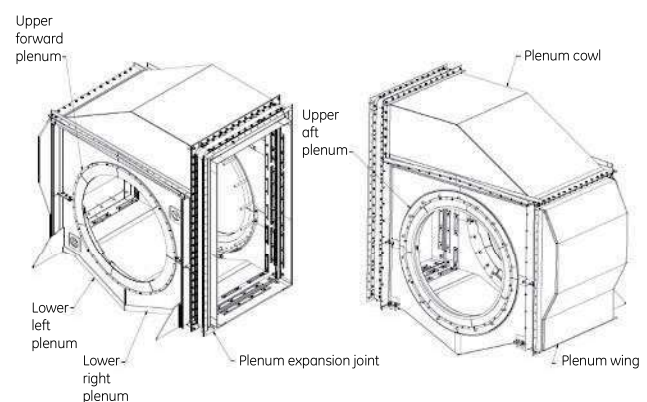
Figure 37. Evolution of 6B plenum from first to second to third (CHROEM) generation.
