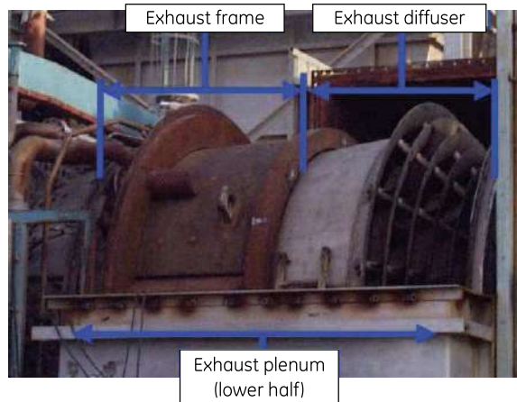
Figure 2. General nomenclature for exhaust components (Frame 9E shown only as an example).
