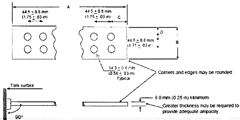
FIGURE 2. Spade Dimensions
