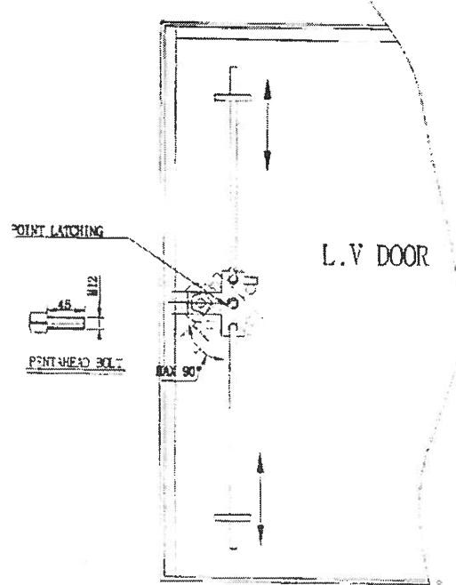
Figure 4 – Three-point latching of Low Voltage Door
